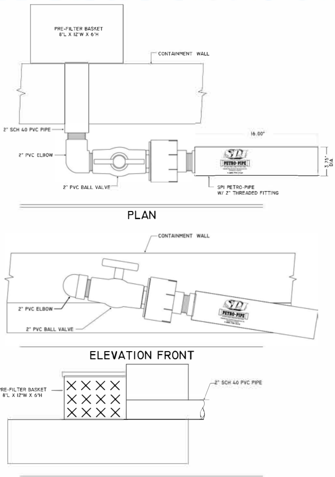
ELEVATION SIDE PIT-416 PETRO-PIPE® W/ PRE-FILTER BASKET
